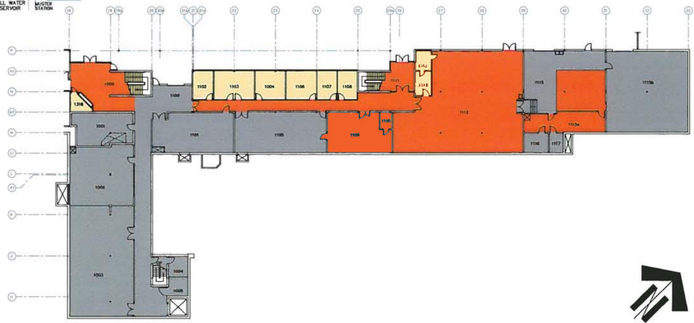
FLOOR PLAN OF ELECTRONICS SHOPS
